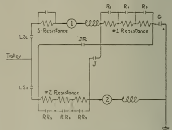
FIG. 3—BRIDGING METHOD CIRCUIT ARRANGEMENTS
